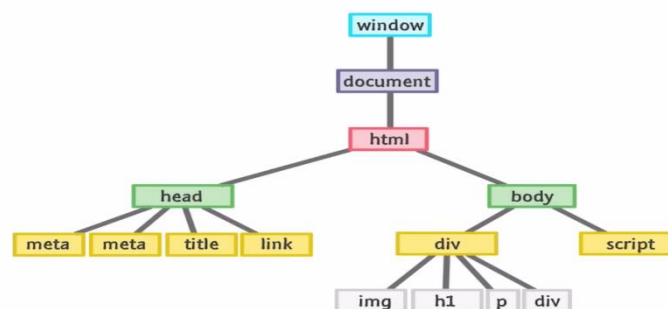
Figure 04: DOM Tree Representation
